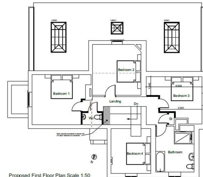
Proposed First Floor Plan Scale 1:50
