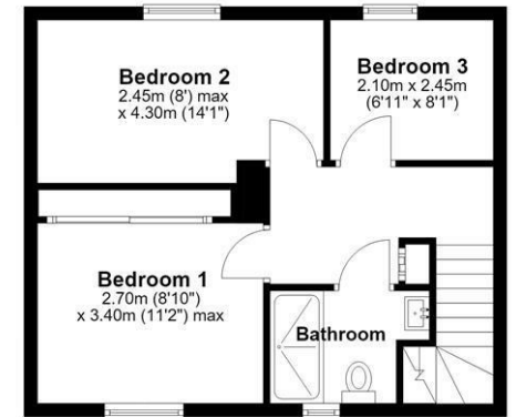
First Floor Approx. 39.4 sq. metres (424.1 sq. feet)
