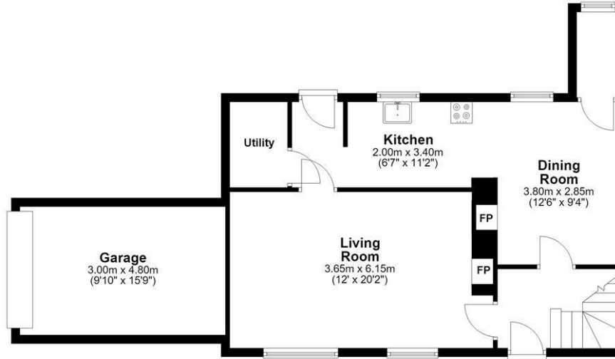
Ground Floor Approx. 69.1 sq. metres (744.1 sq. feet)
